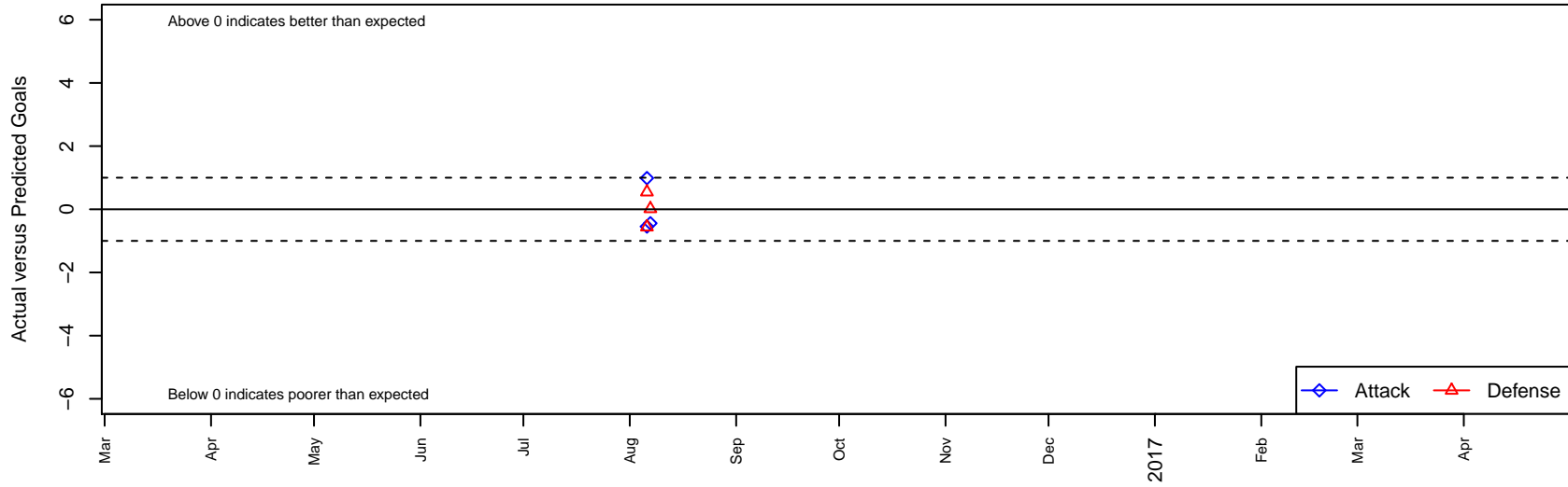
Beach FC LB Arrache G04 Dots are actual minus expected GF (blue circles) and GA (red triangles). Blue line is smoothed change in attack strength. Red is smoothed change in defense strength.
